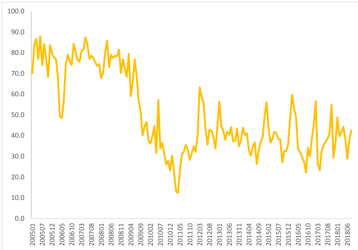
Figure 5.1.: The average value of Transparency Index (TI) by months from January 2005 to August 2018, N = 193,661, %
