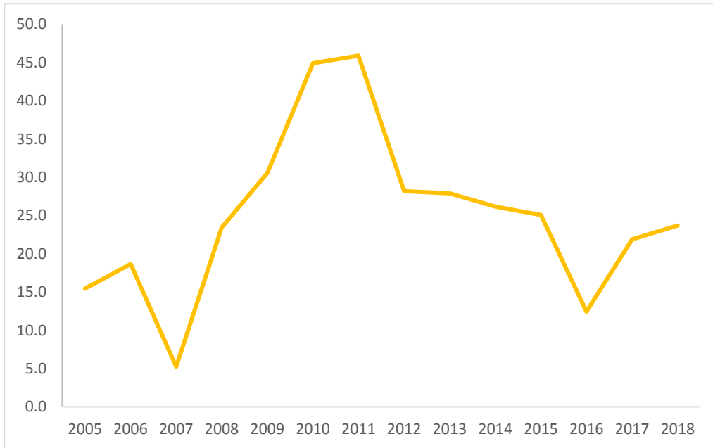
Figure 3.2: Share of contracts financed by EU by years, from January 2005-to August 2018, N = 193,661, %
