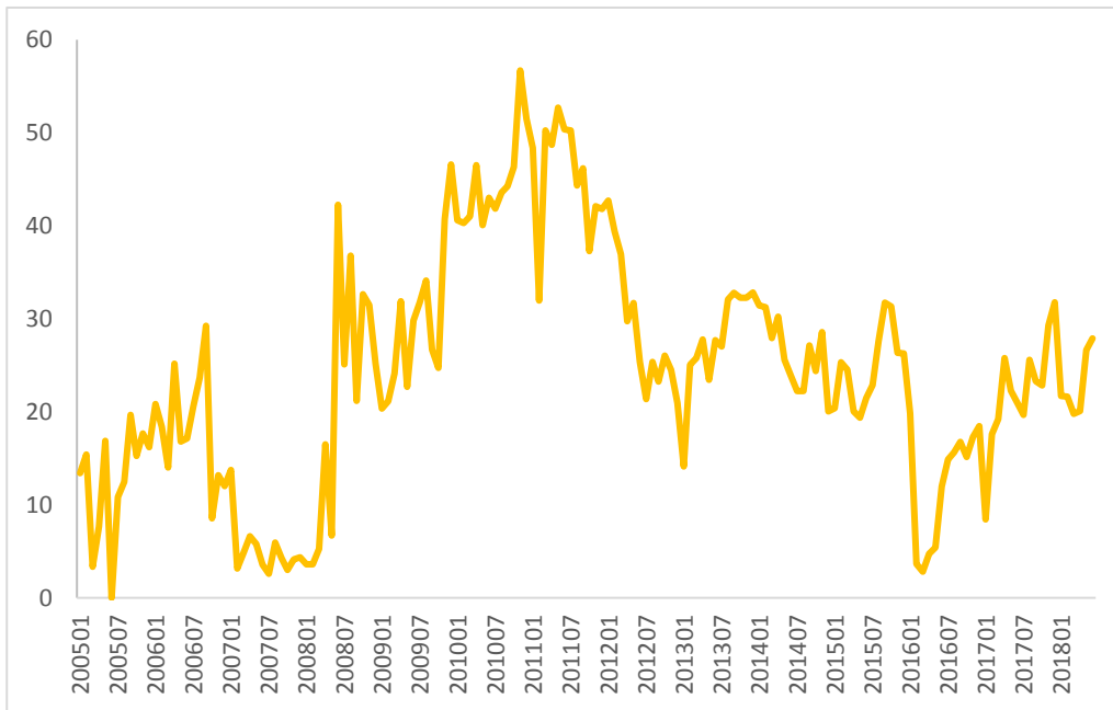
Figure 3.1.: Share of contracts financed by EU by months, from January 2005- to August 2018, N = 193,661, %
