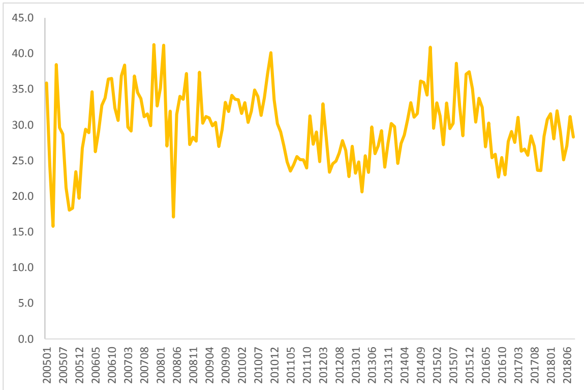
Figure 6.1. Share of contracts without competition (single-bidder, SB) in total number of contracts by months, from January 2005 to August 2018, N = 190,367, %
