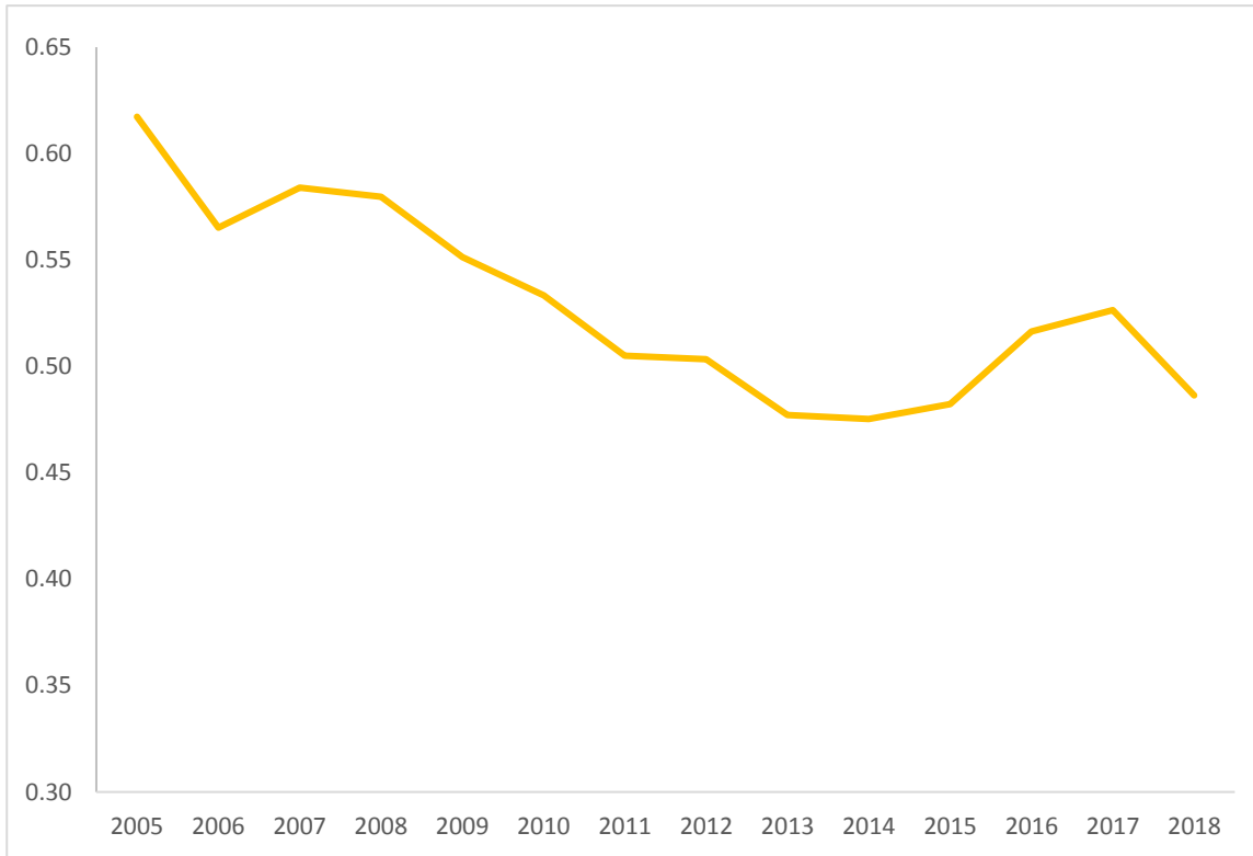
Figure 4.2.: The average value of ICI by years, from January 2005 to August 2118, N = 131,888, %
