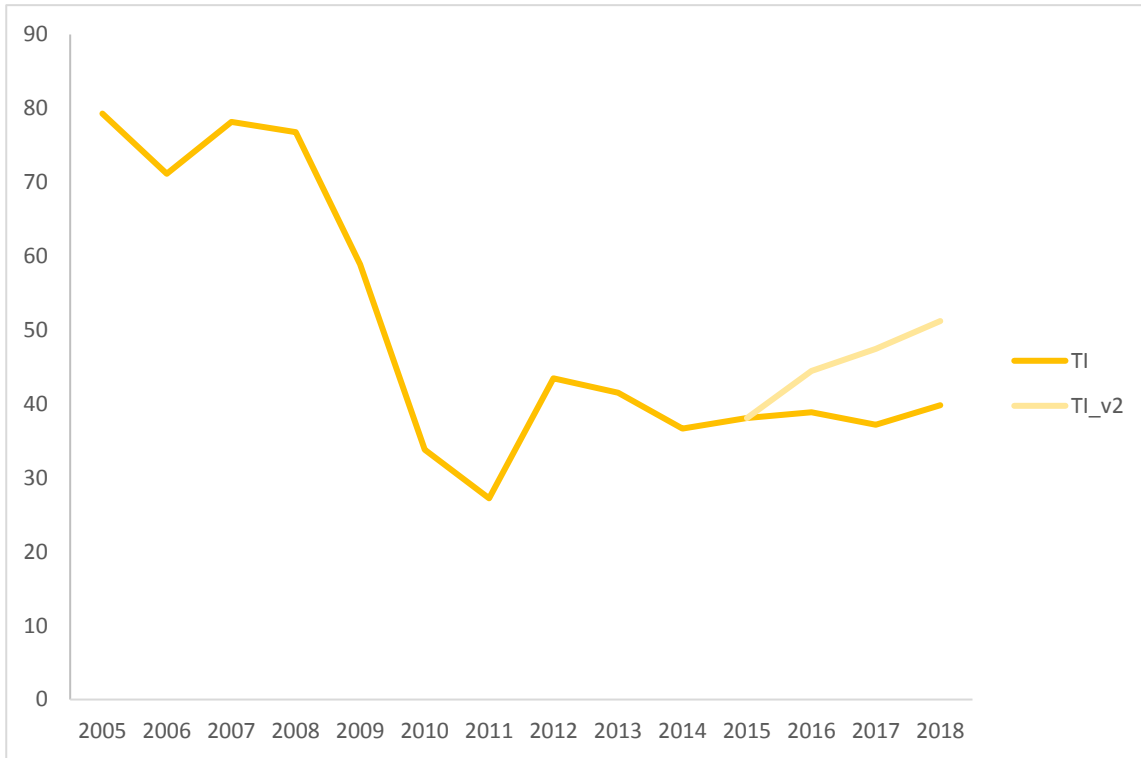
Figure 5.2.: The average value of Transparency Index (TI) and TI_v2 by years from January 2005 to August 2018, N = 193,661, %
