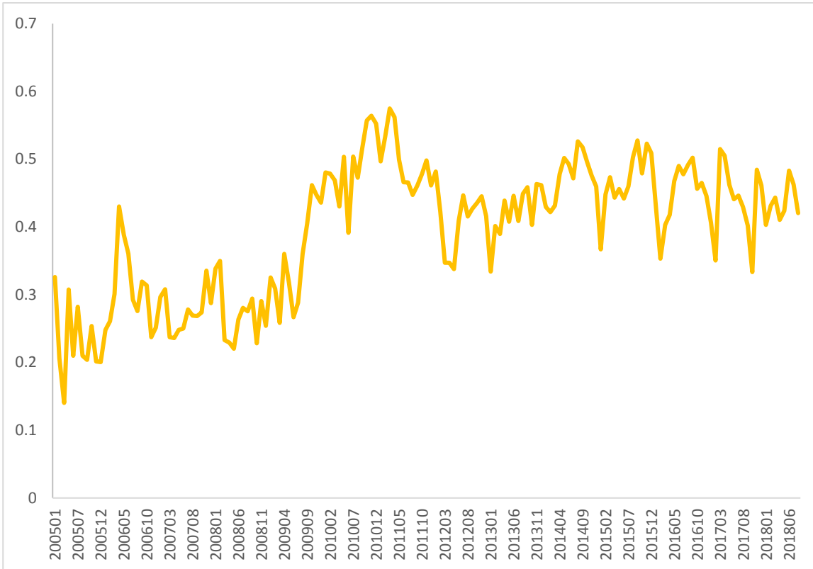
Figure 7.1.: The Corruption Risk Indicator (CR2) in Hungarian public procurement, from January 2005 to August 2018, monthly data, N = 190,367
