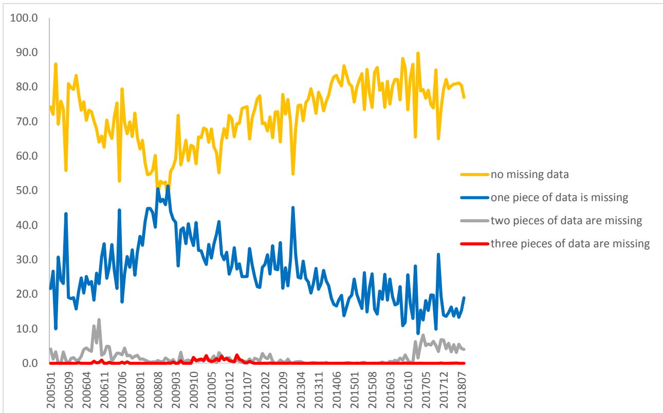
2.1. Figure: Average share of contract award notices with missing data by months (indicators a1-a4), from January 2005 to August 2018, N = 193,661, %
