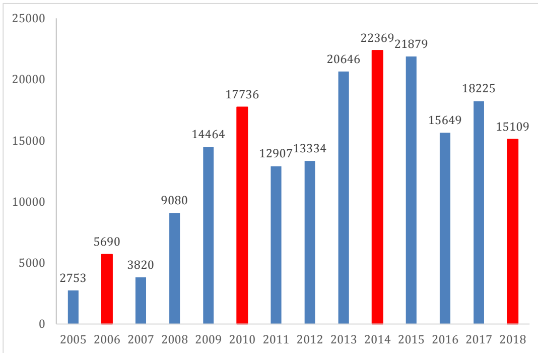
Figure 1.1.: Number of contracts from January 2005 to August 2018, N = 193,661, without framework agreements
