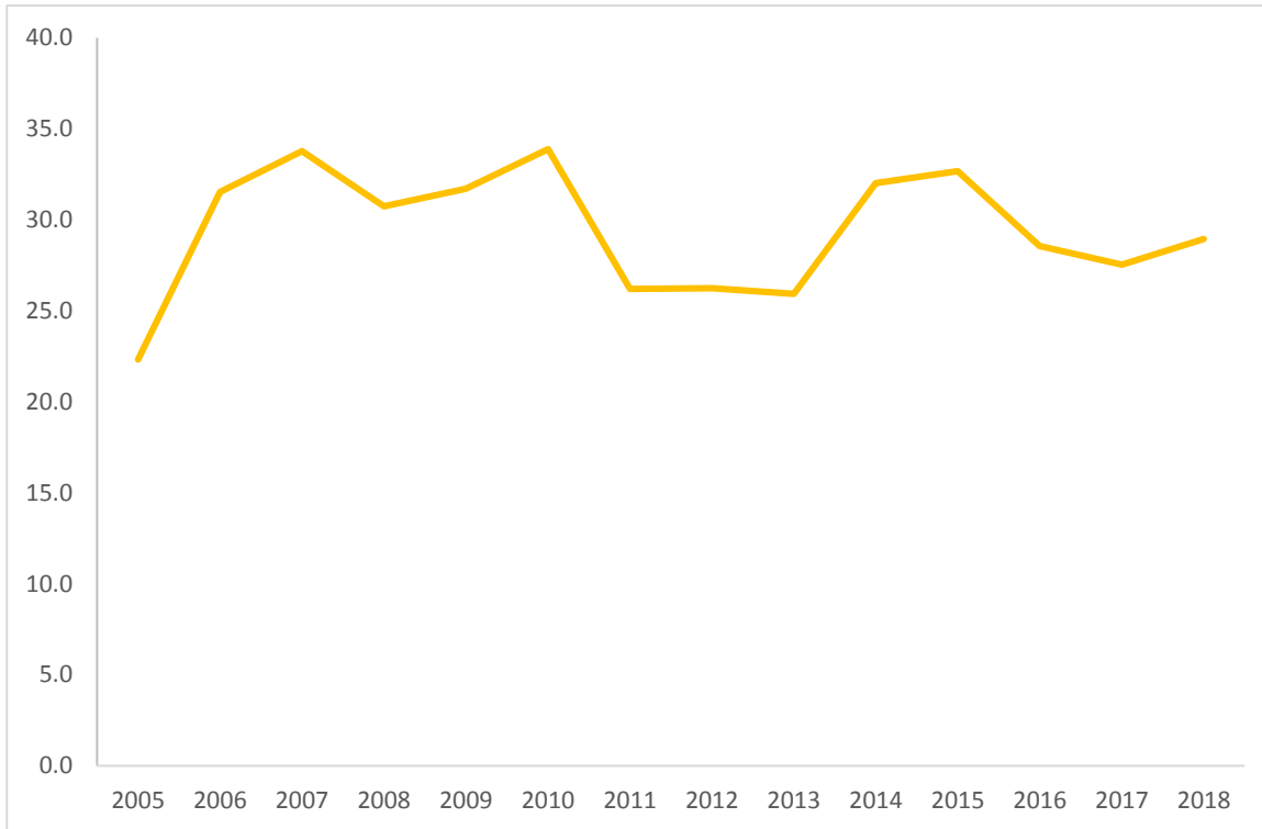
Figure 6.2.: Share of contracts without competition (single-bidder, SB) in total number of contracts by years, from January 2005 to August 2018, N = 190,367, %
