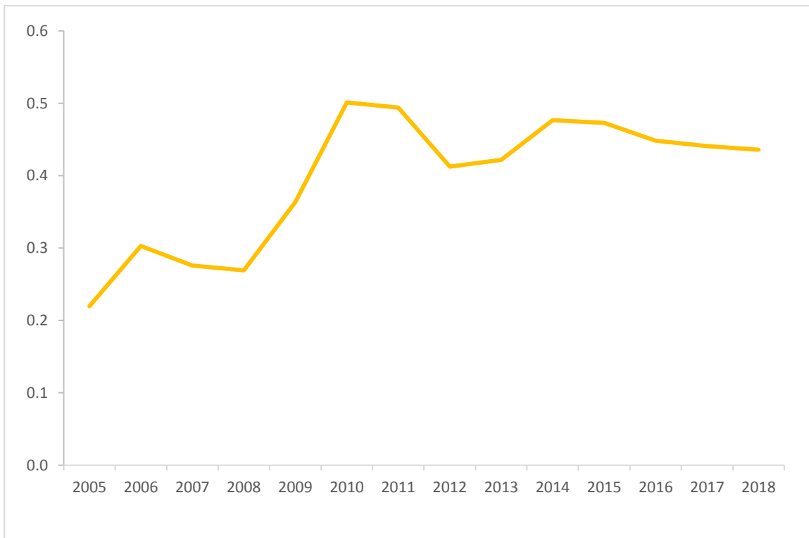
Figure 7.2.: The Corruption Risk Indicator (CR2) in Hungarian public procurement, from January 2005 to August 2018, yearly data, N = 190,367
