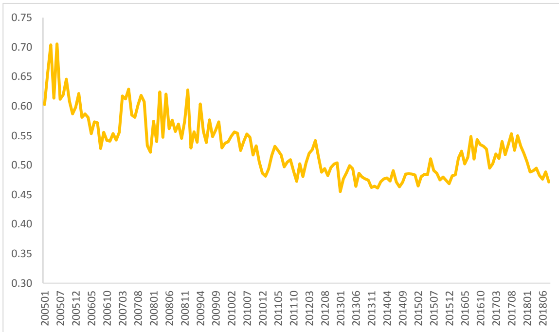
Figure 4.1.: The average value of ICI by months, from January 2005 to August 2118, N = 131,888, %
